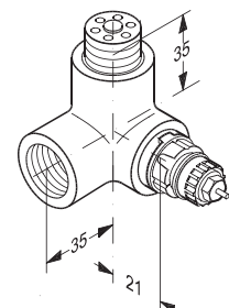
return valve
