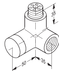
lockshield valve
