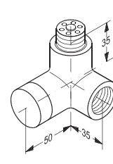
lockshield valve
