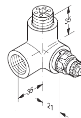
return valve
