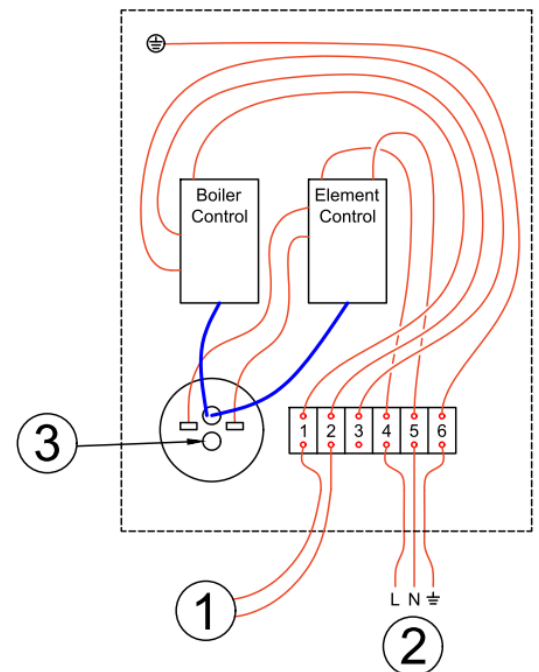
Twin Coil Cylinder: Heat Source Without Probe
