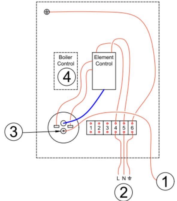
Twin Coil Cylinder: Heat Source with Probe
